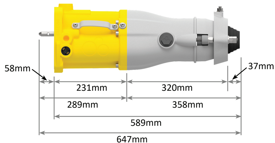
Side View (ARM)
