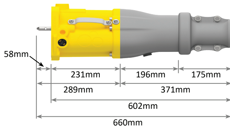
Side (UN-ARM)
