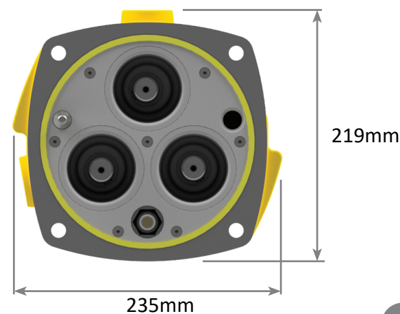
Front View with Live Line Indicators
