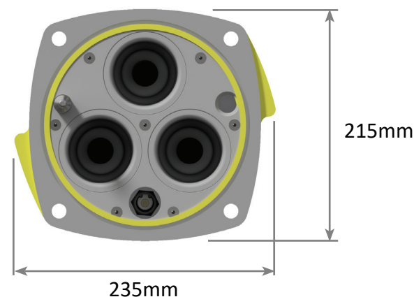
Front View without Live Line Indicators
