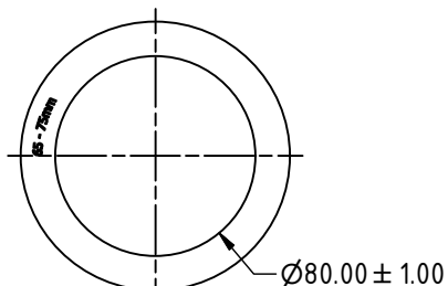
CABLE COMPRESSION WASHER
