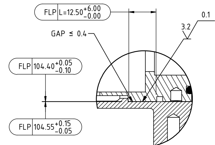
FLAMEPATH DETAIL C
