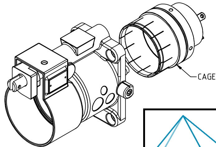
ASSEMBLY
