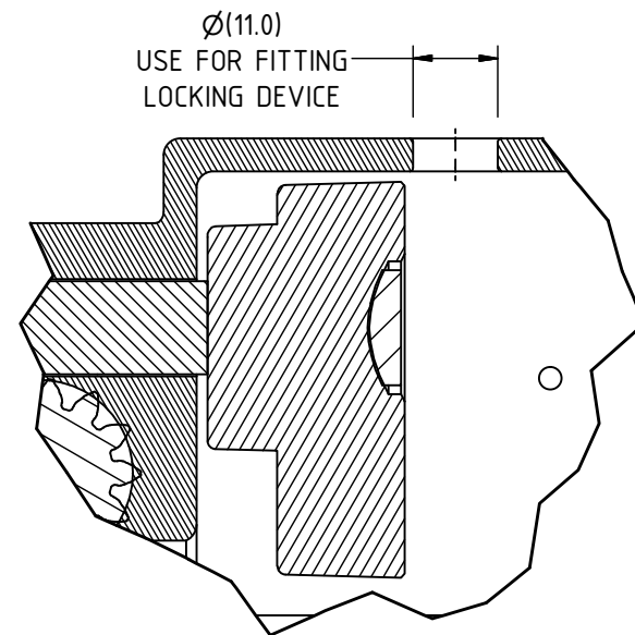
DETAIL FOR LOCKING DEVICE LOCATION
