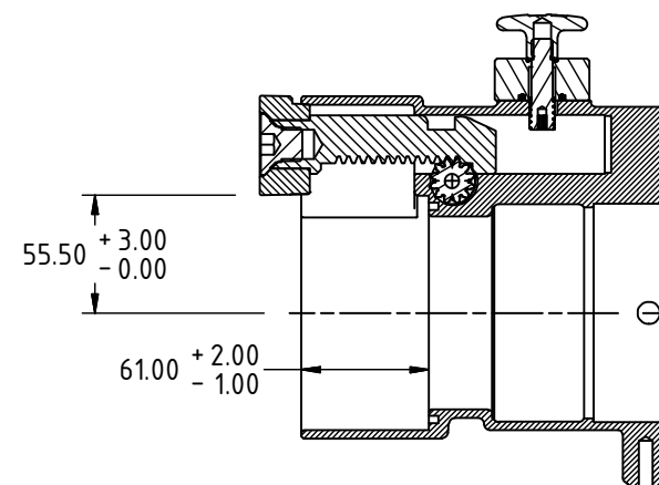
SECTION C-C
