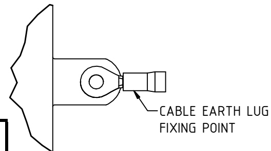
DETAIL D
