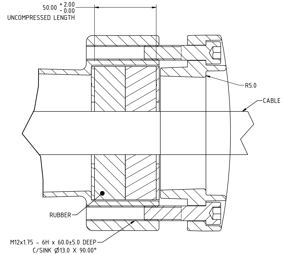
CABLE ENTRY DETAIL
