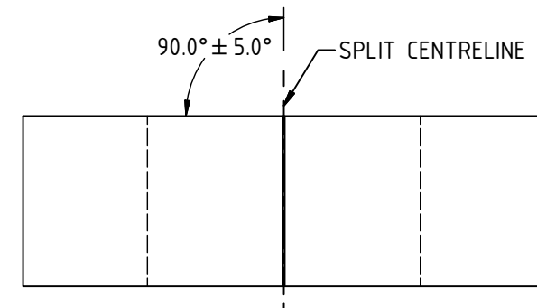
SIDE VIEW COMPRESSION GLAND RUBBER
