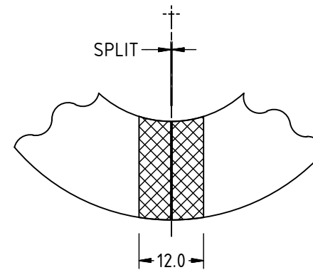
DETAIL 1
