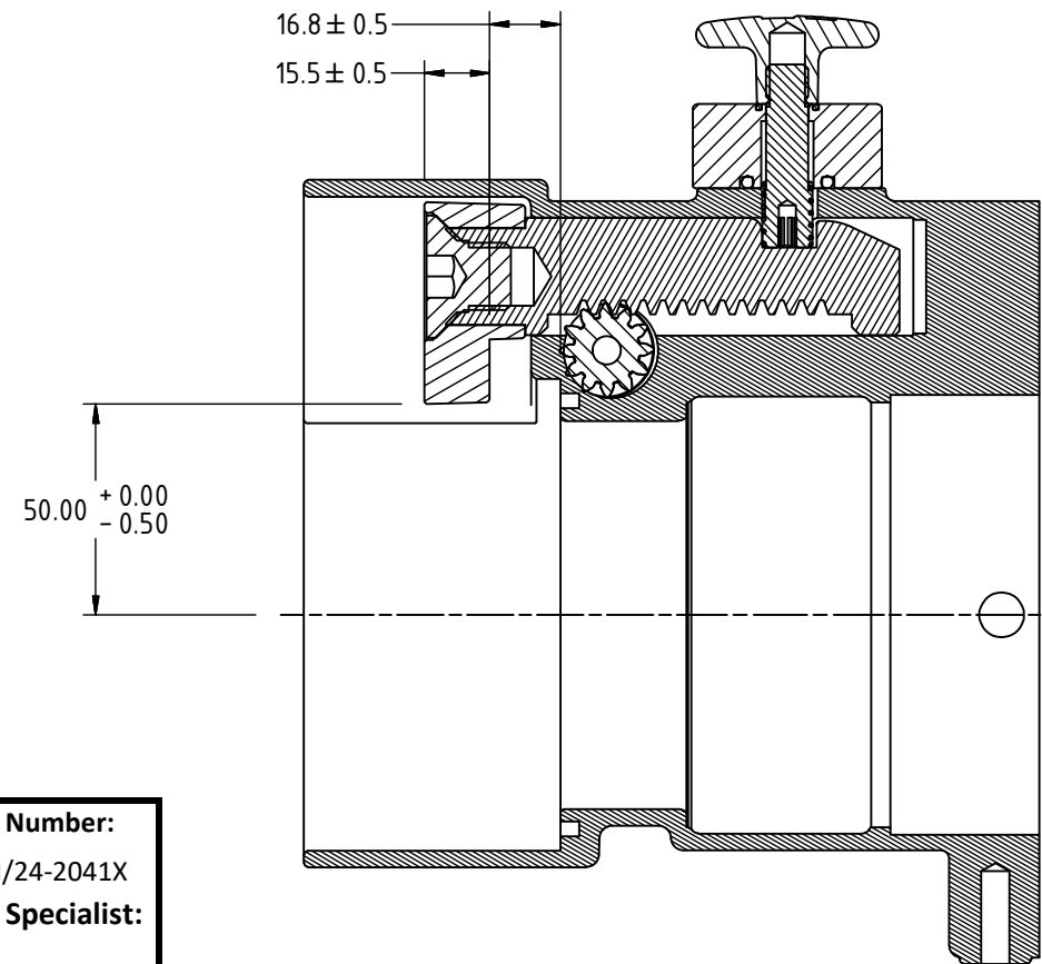
SOCKET SECTION VIEW
