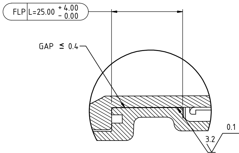
PLUG SOCKET ENGAGEMENT FLAMEPROOF PATH DETAIL B
