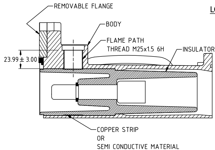
SECTION VIEW LIVE LINE INDICATOR
