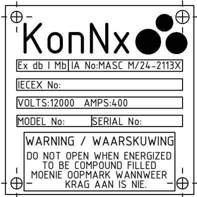
END COVER PRODUCT DATA LABEL
