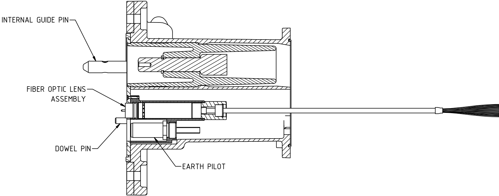
SECTION EV-EV
