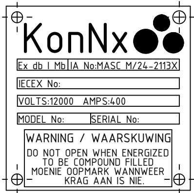
R/F L/L F/O BODY PRODUCT DATA LABEL
