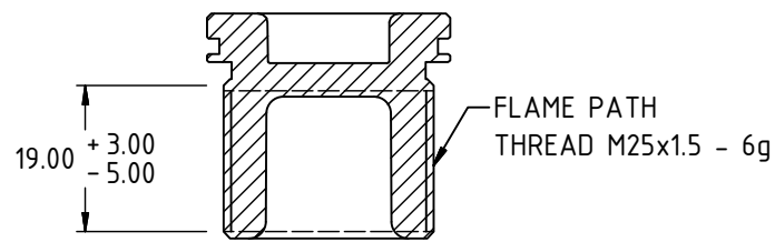
SECTION C-C LIVE LINE BUNG
