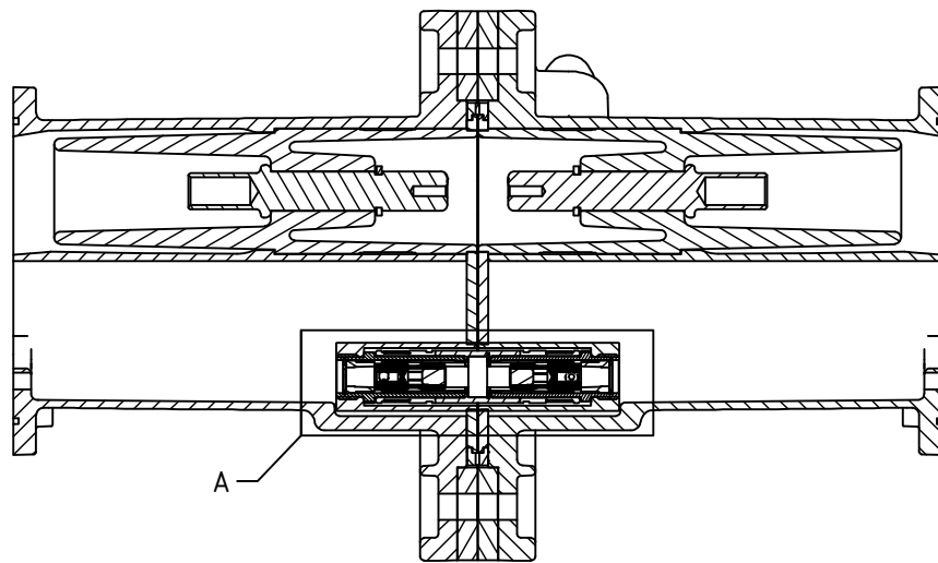
SECTION VIEW COUPLER WITH EARTH PILOT CONNECTION
