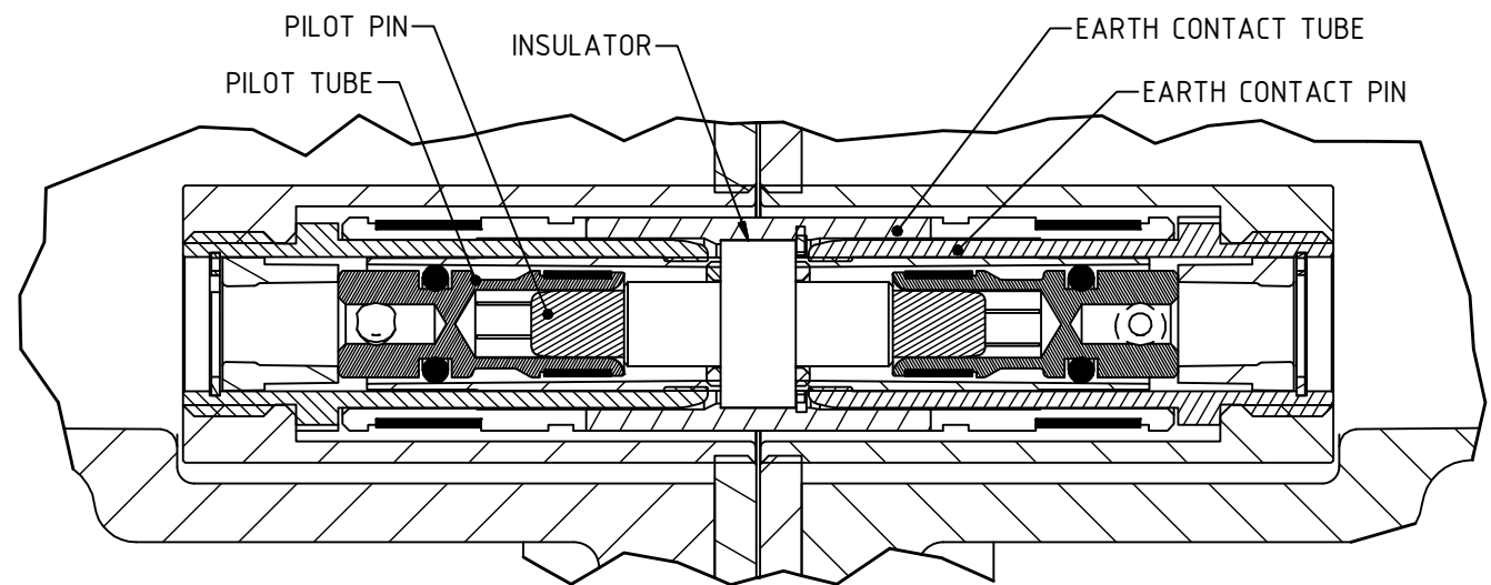
SECTION VIEW EARTH PILOT CONNECTION
