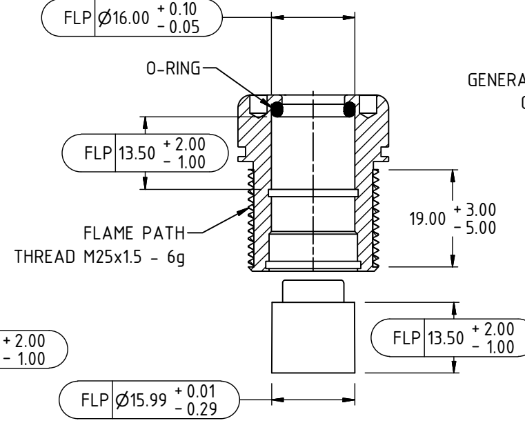
SECTION A-A LOW PROFILE LIVE LINE INDICATOR ASSEMBLY
