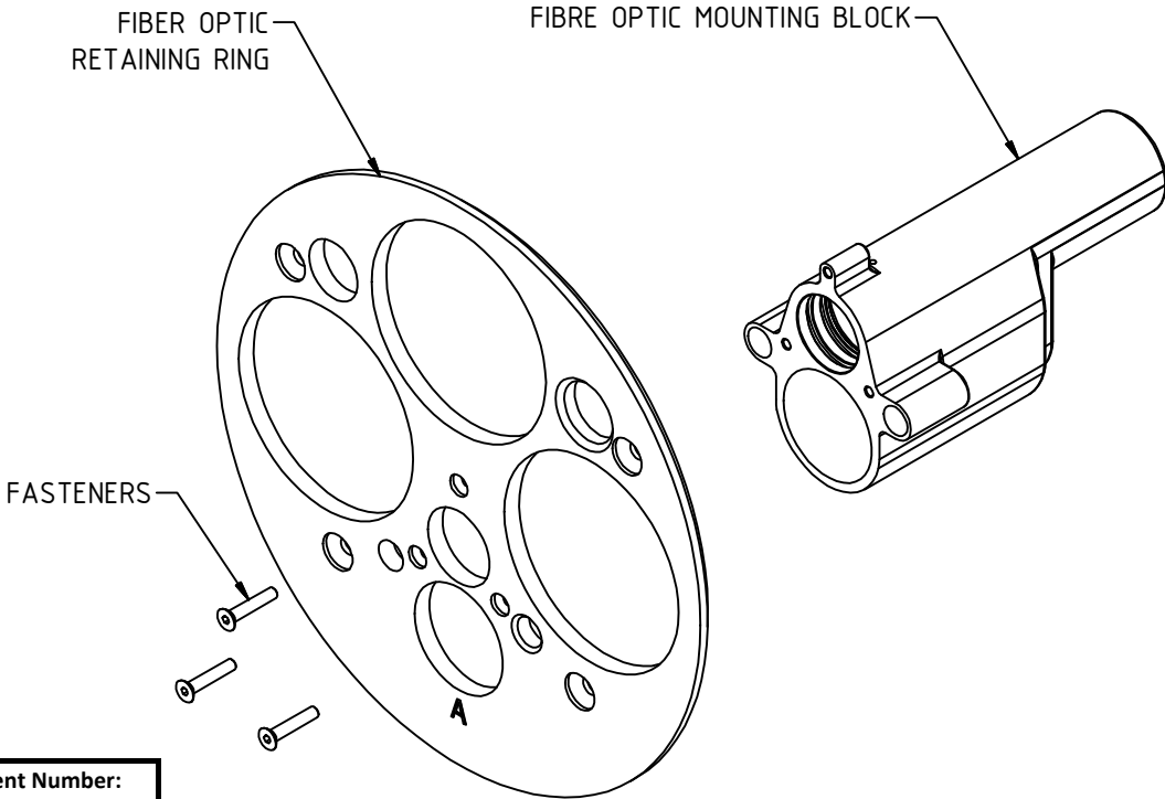
EXPLODED VIEW RETAINING RING WITH FIBER OPTIC MOUNT
