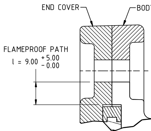
SECTION A-A FLAMEPROOF PATH DETAIL
