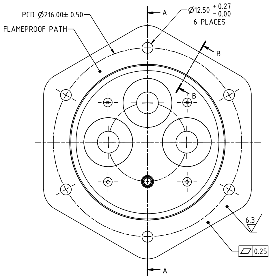
REAR VIEW END COVER
