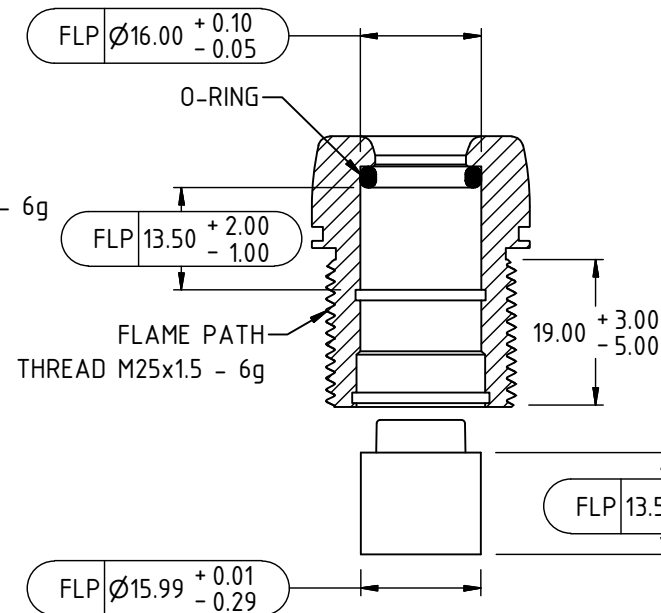
SECTION D-D LOW PROFILE LIVE LINE INDICATOR ASSEMBLY WITH IMPACT PROTECTION
